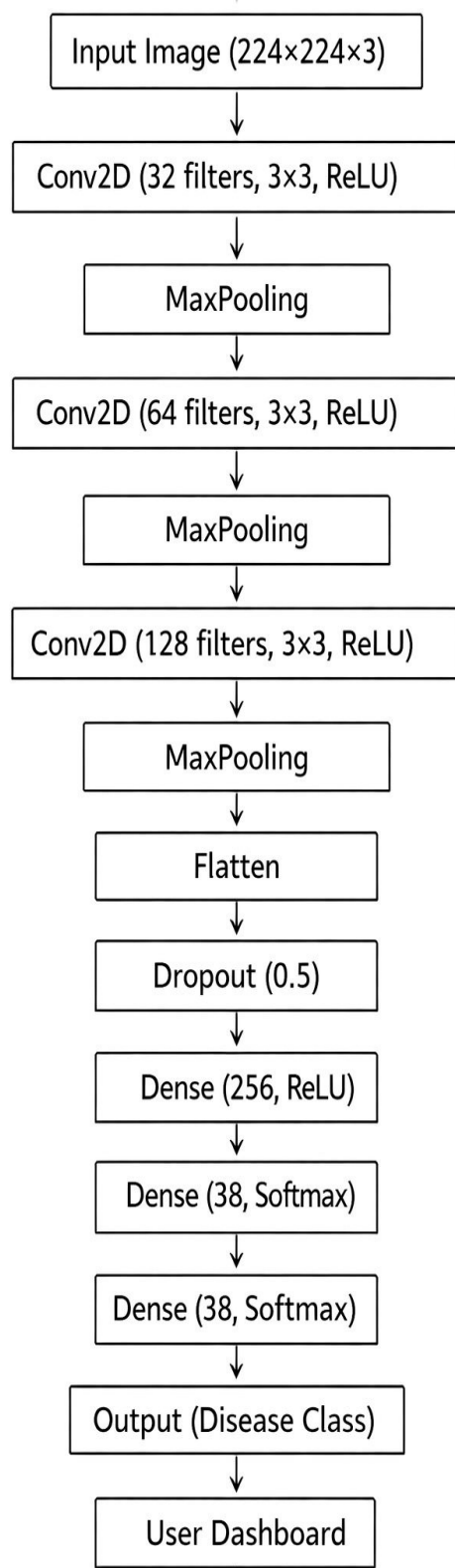
Fig. 5.1: CNN Architecture for Plant Disease Classification
